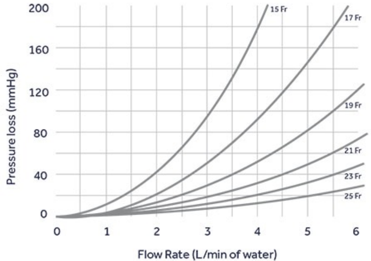
Pressure Loss Across ARTERIAL 15-25Fr Cannula
